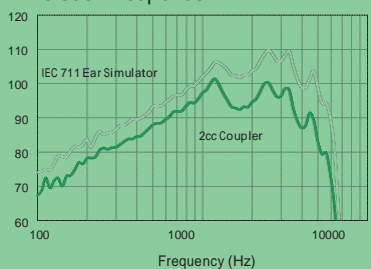
Input/Output Response
