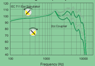
Basic frequency response and effect of High Frequency Cut
