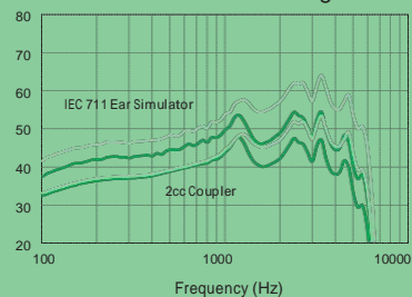
Full-on and Reference test gain
