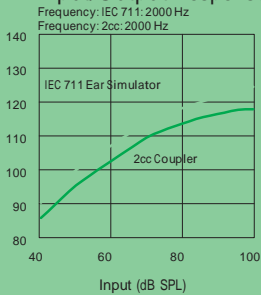
Input/Output Response
